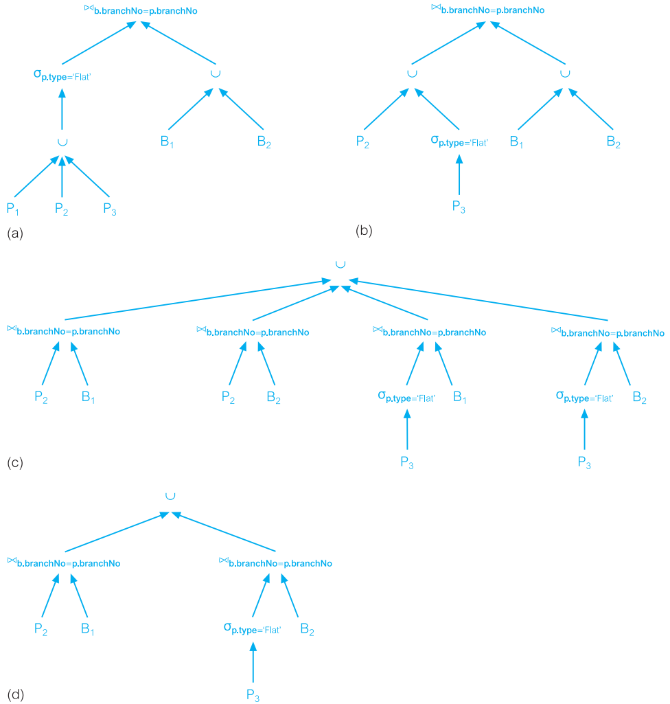
Figure 23.17 Relational algebra trees for Example 23.2: (a) generic tree; (b) tree resulting from reduction by selection; (c) tree resulting from commuting join and union; (d) reduced tree.
